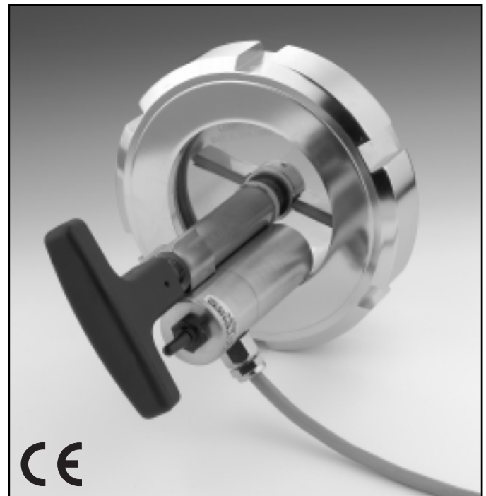
Lumiglas Stainless Steel Mini-Luminaire, Series USL 01 with mounting clamp fitted on a screwed sightglass fitting with Lumiglas sightglass wiper type SW I.
